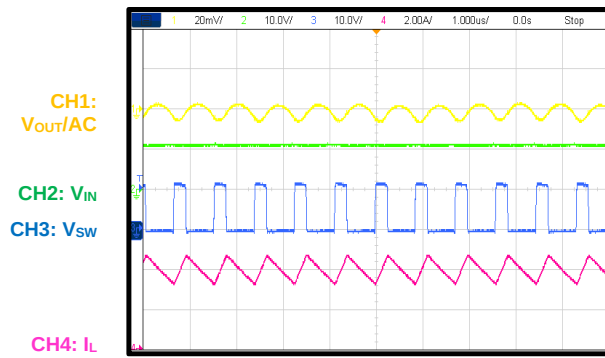
Output Ripple
