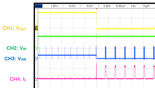
Short-Circuit Entry
