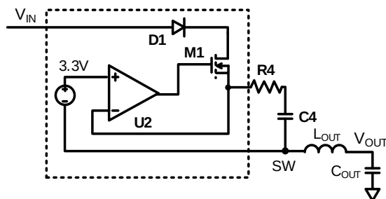
Figure 5: Internal Bootstrap Charger
