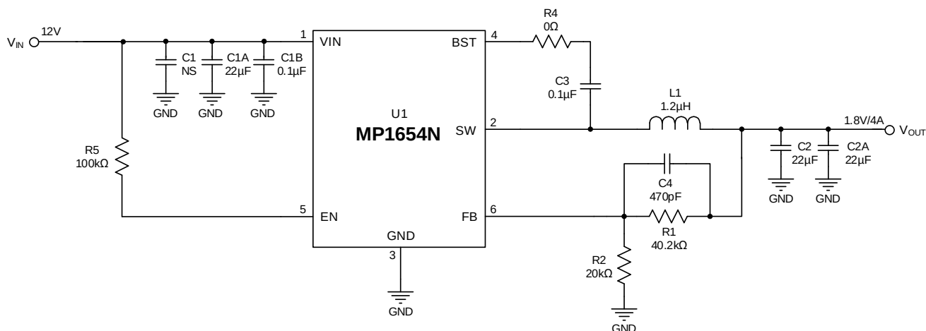
Figure 11: Typical Application Circuit ( V_{IN} = 12V , V_{OUT} = 1.8V/4A )
