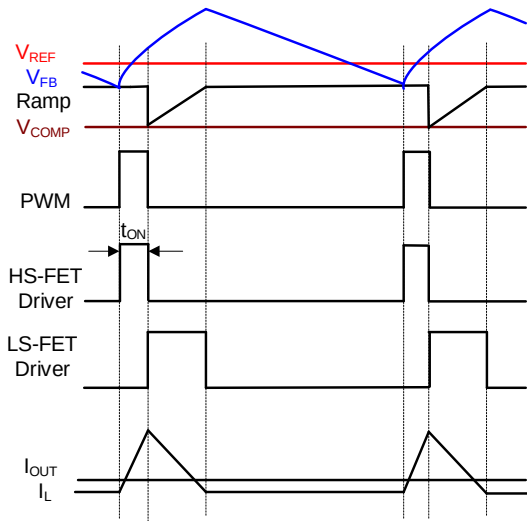
Figure 4: Power-Save Mode at Light Loads
