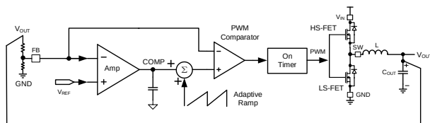
Figure 2: COT Control
