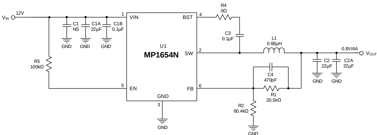
Figure 15: Typical Application Circuit ( V_{IN} = 12V , V_{OUT} = 0.8V/4A )
