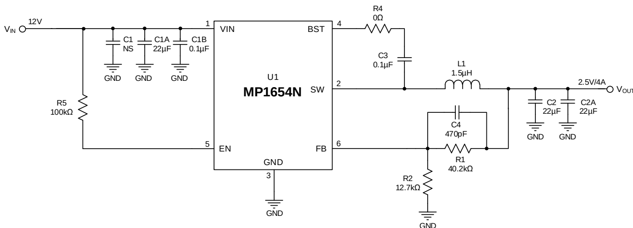
Figure 10: Typical Application Circuit ( V_{IN} = 12V , V_{OUT} = 2.5V/4A )
