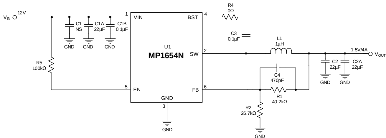
Figure 12: Typical Application Circuit ( V_{IN} = 12V , V_{OUT} = 1.5V/4A )
