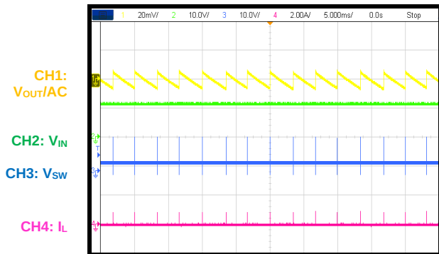
Output Ripple
