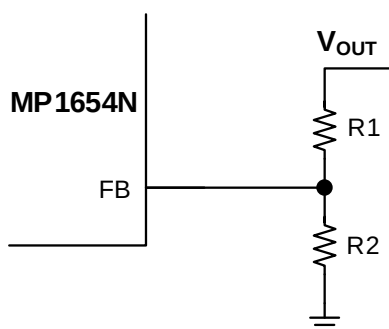
Figure 6: Feedback Network
