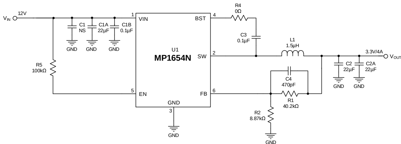
Figure 9: Typical Application Circuit ( V_{IN} = 12V , V_{OUT} = 3.3V/4A )
