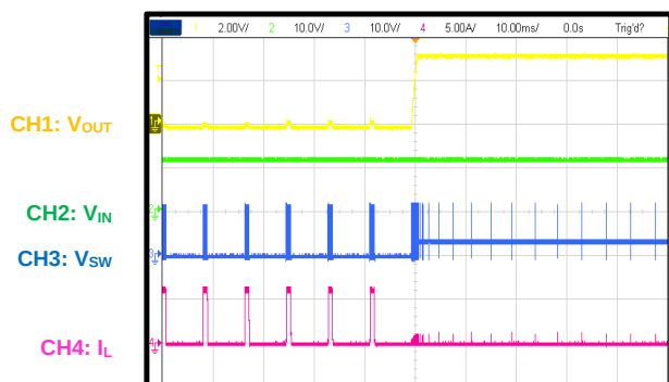
Short-Circuit Recovery
