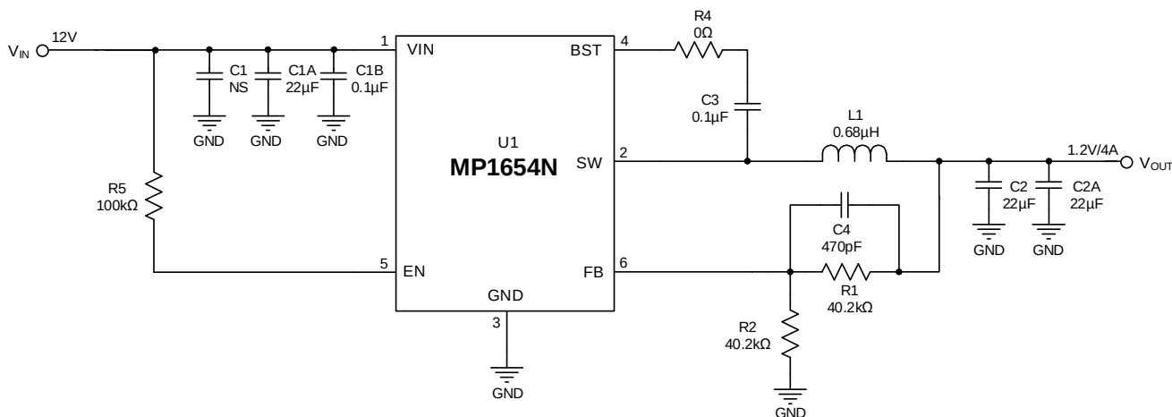
Figure 13: Typical Application Circuit ( V_{IN} = 12V , V_{OUT} = 1.2V/4A )
