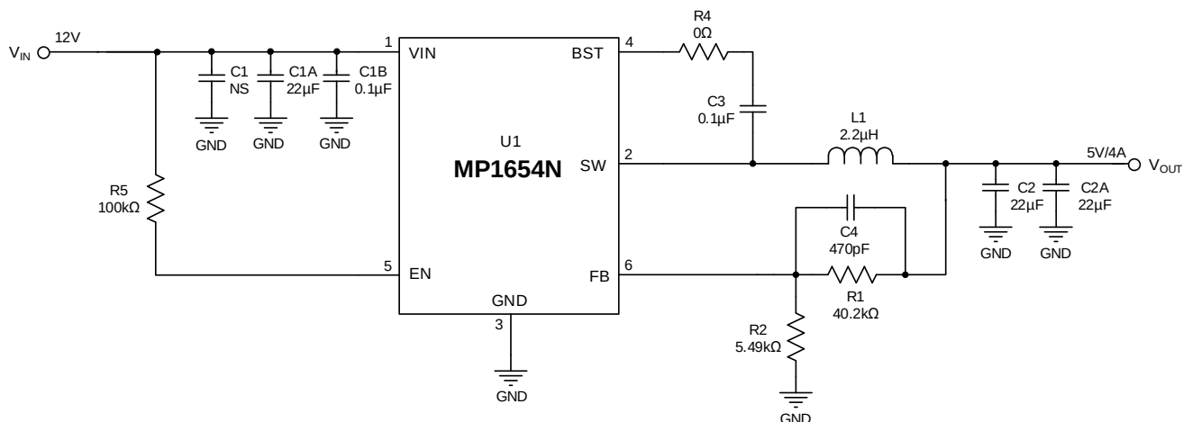
Figure 8: Typical Application Circuit ( V_{IN} = 12V , V_{OUT} = 5V/4A )
