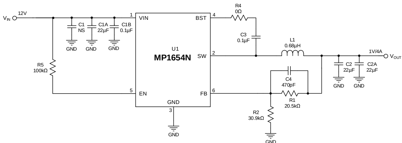
Figure 14: Typical Application Circuit ( V_{IN} = 12V , V_{OUT} = 1V/4A )
