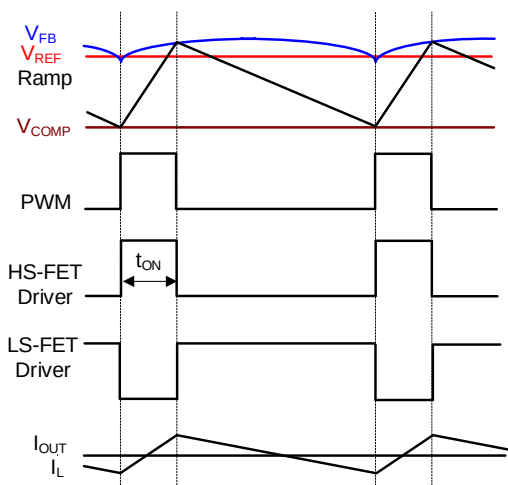
Figure 3: Heavy-Load Operation
