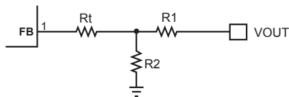
Figure 6— T-type Network
