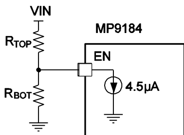
Figure 2: VIN UVLO Program
