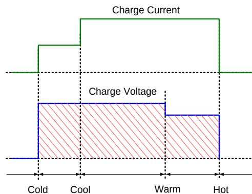
Figure 7: NTC Window under JEITA Control
