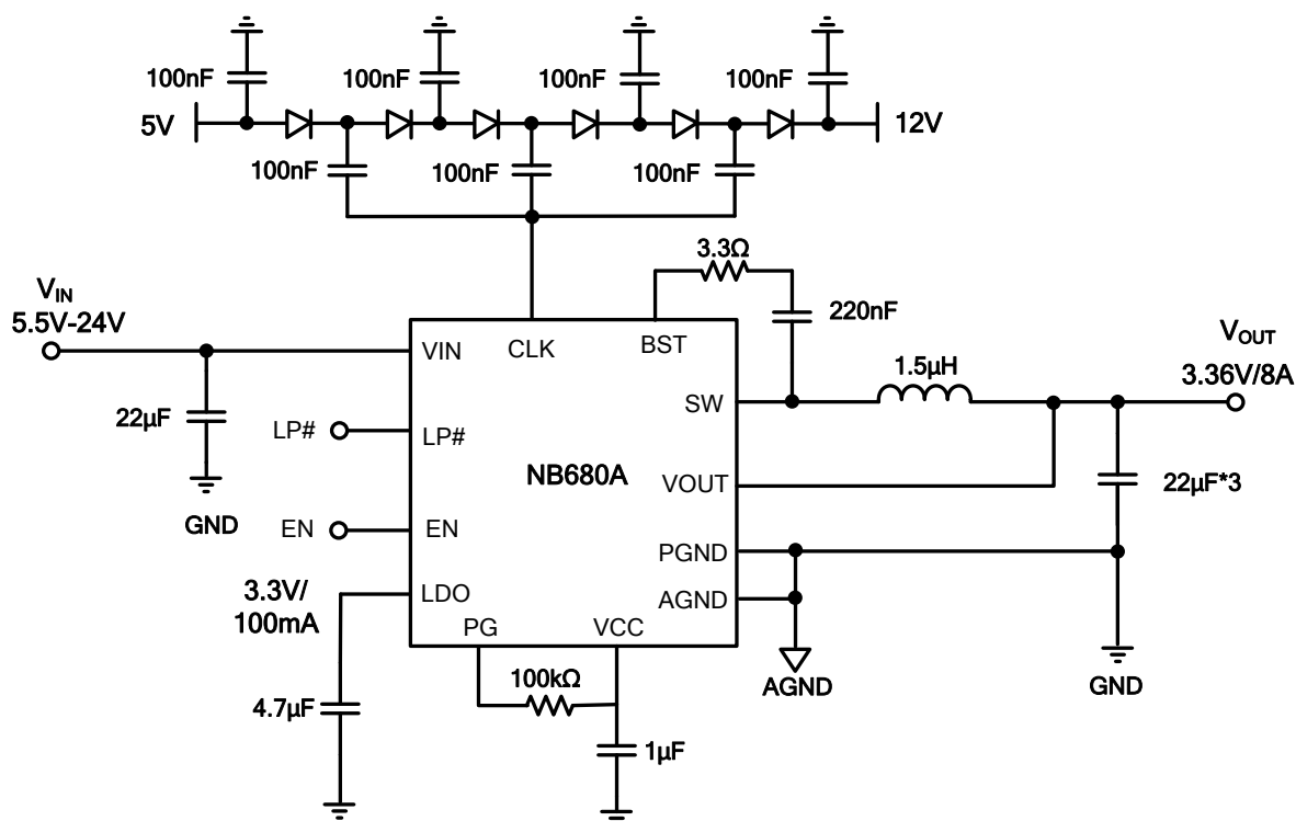
Figure 8: Typical Application Schematic with Ceramic Output Capacitors
