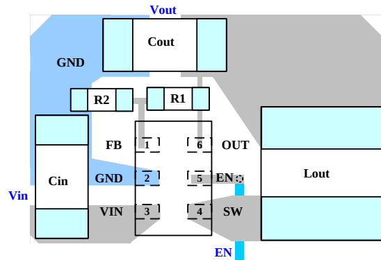
Figure 3: Two Ends of Input Decoupling Capacitor Close to Pin 2 and Pin 3
