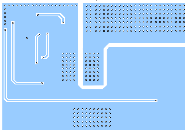
Inner 2
