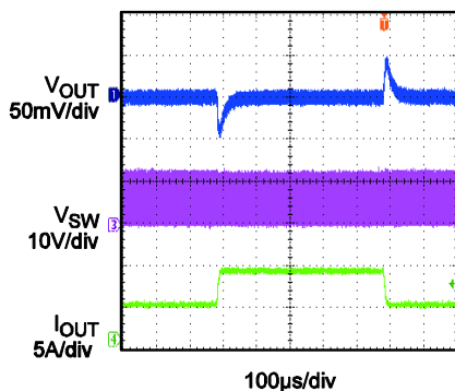
Load Transient Response I_{OUT} = 4A \rightarrow 8A, 1A/\mu s
