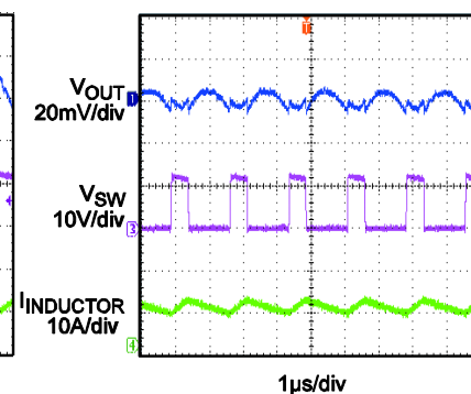
Output Ripple Voltage I_{OUT} = 8A
