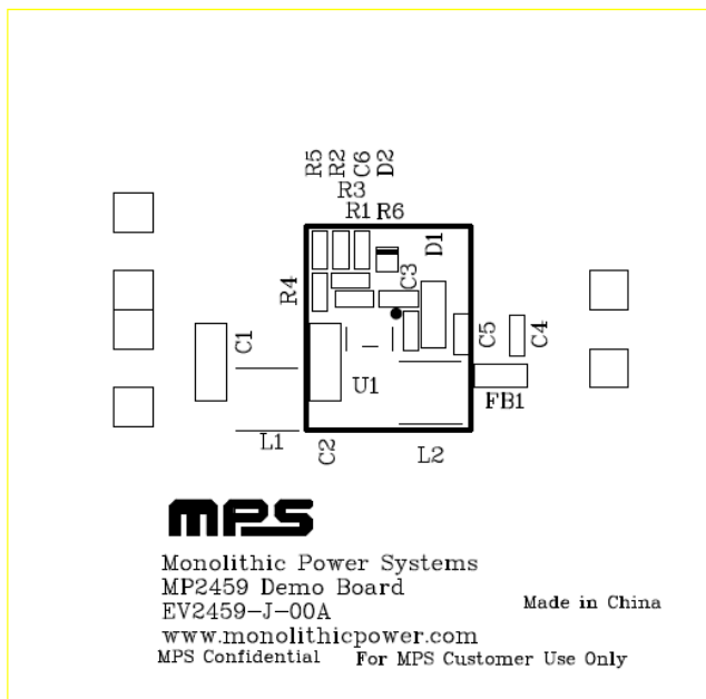
Figure 3—Top Silk
