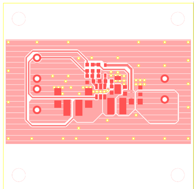
Figure 4- Top Layer
