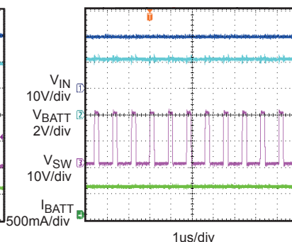
Steady State Waveform
