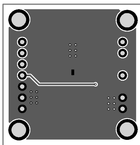
Figure 4: Bottom Layer
