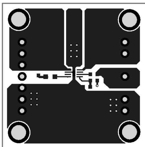
Figure 3: Top Layer
