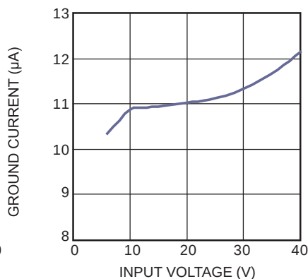
Ground Current vs. V_{IN} I_{OUT}=0mA
