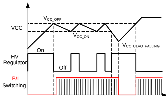
Figure 4: Start-Up and UVLO Operation
