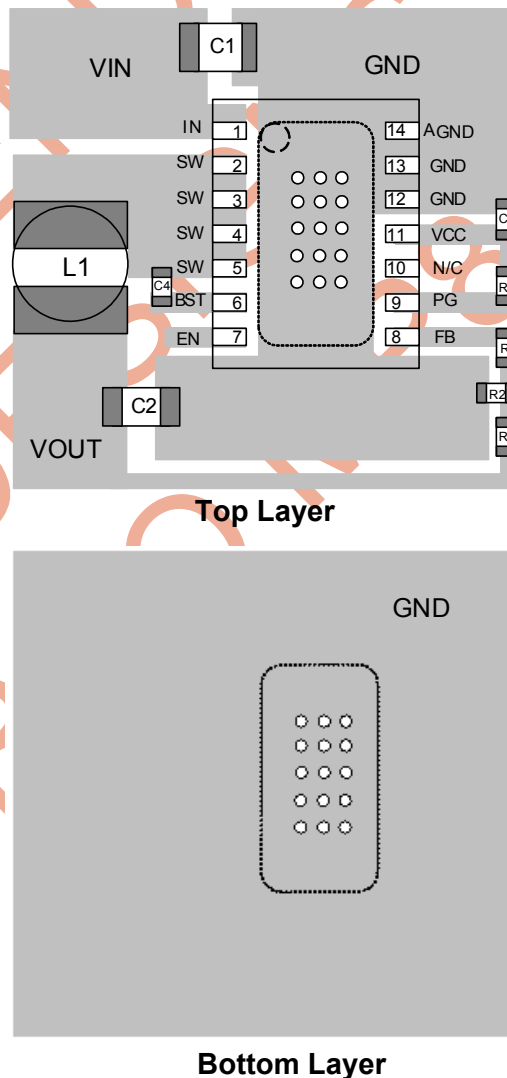
Figure 7—PCB Layout
