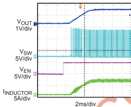
Enable Startup with 6A Load
