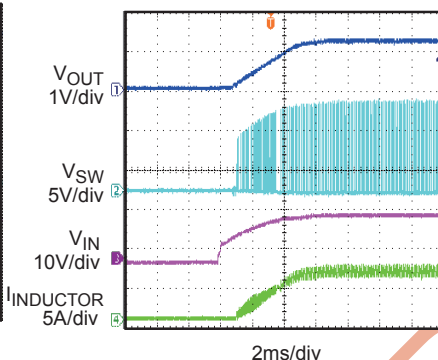
Power up with 6A Load
