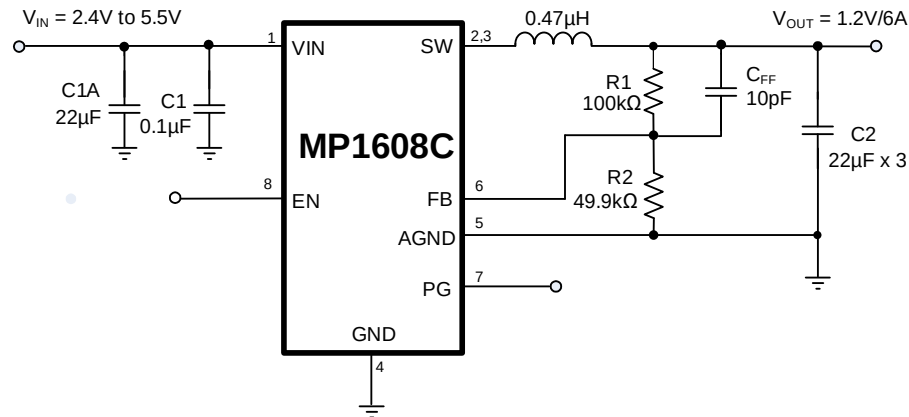
Figure 5: Typical Application Circuit ( V_{IN} = 2.4V to 5.5V , V_{OUT} = 1.2V/6A )
