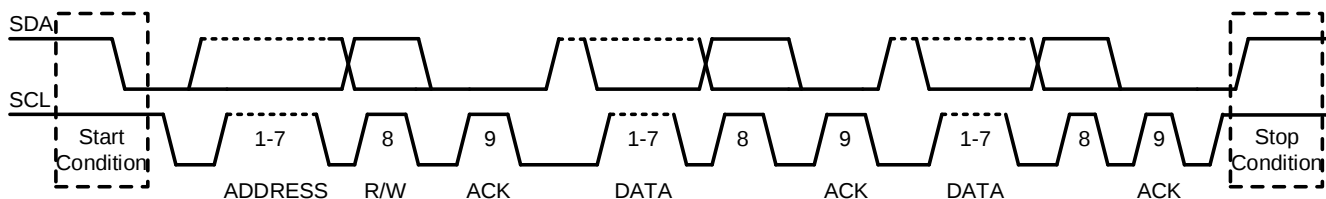
Figure 15: Complete Data Transfer
