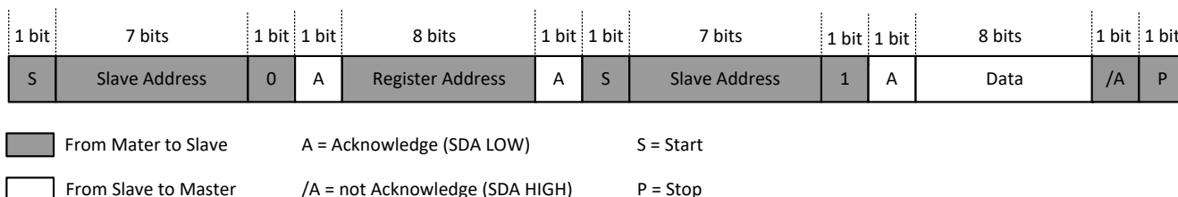
Figure 17: I²C Single Read
