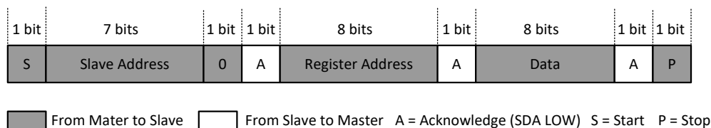
Figure 16: I²C Single Write
