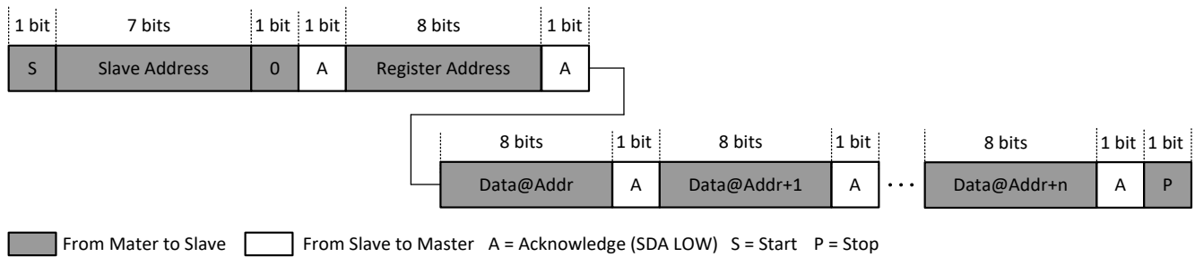
Figure 18: I 2 C Multi-Write
