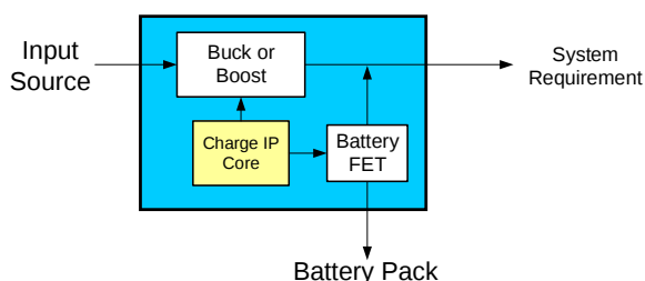
Figure 7: NVDC Power Path Management Structure
