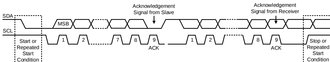
Figure 14: Data Transfer on the I²C BUS
