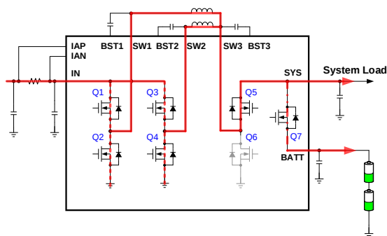
Figure 3: Power MOSFETs' State in Buck Charging Mode
