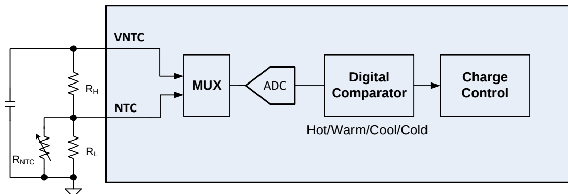
Figure 22: Temperature Sensing
