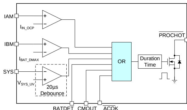
Figure 11: PROCHOT Events
