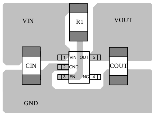
Figure 3—MP2009 Top Layer
