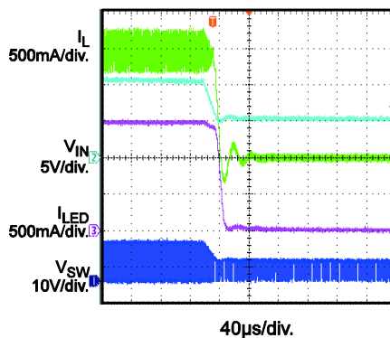
V_{IN} Shutdown
