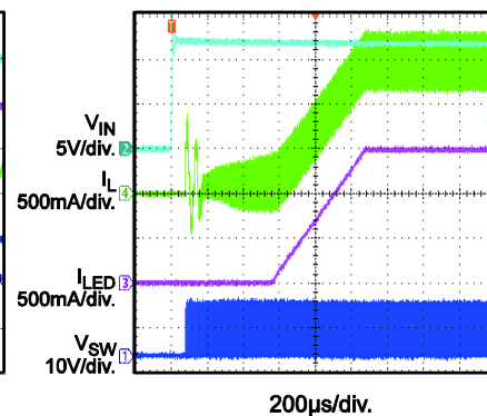
V_{IN} Start-Up
