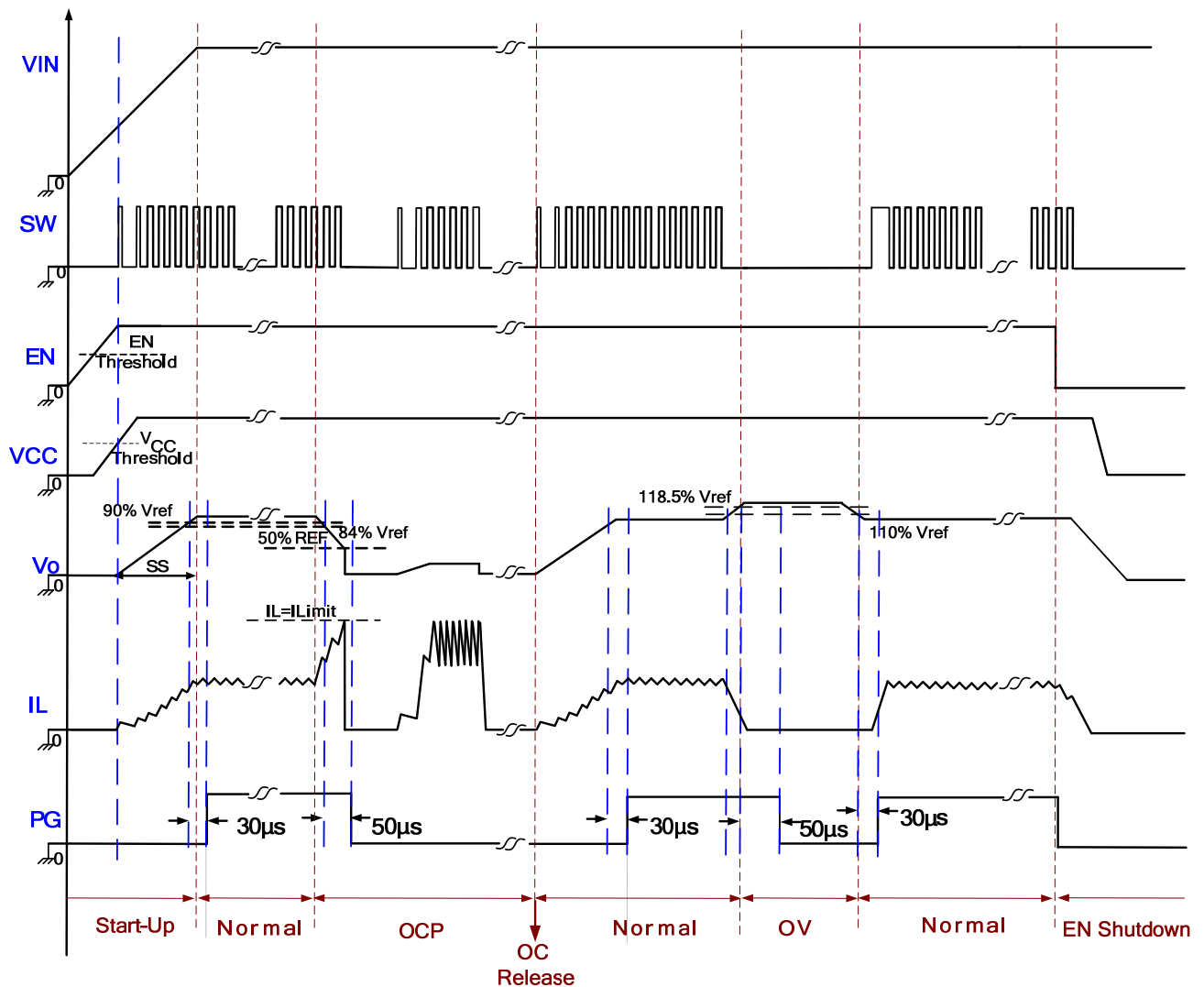
Figure 2: Timing Sequence
