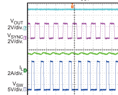
SYNC Operation (180° Out-of-Phase)
