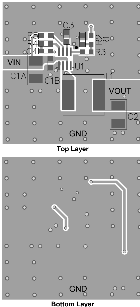
Figure 7: Recommended PCB Layout
