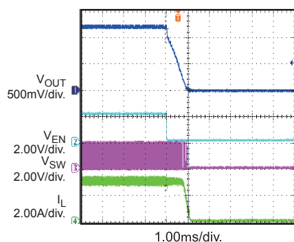
EN Shut Down with 3A Load
