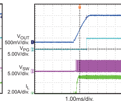
Power Good On with 3A Load
