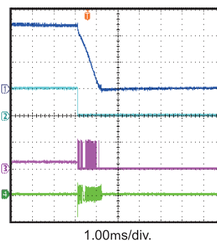
EN Shut Down without Load
