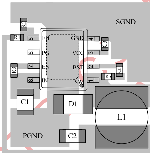
Figure 3—PCB Layout for Single Layer
