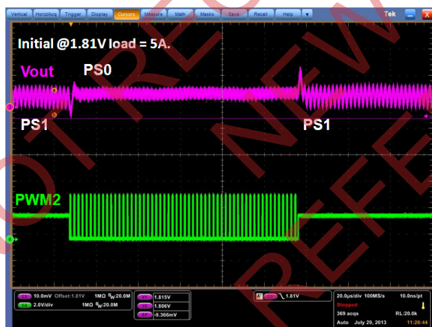
FIGURE 5(a). 1-Phase CCM → 6-Phase → 1-Phase CCM
