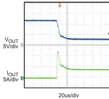
0.66 \Omega Load Connected to Enabled Device
