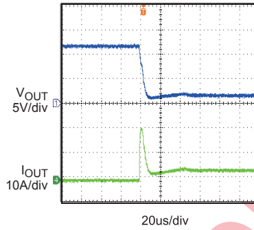
0.33 \Omega Load Connected to Enabled Device
