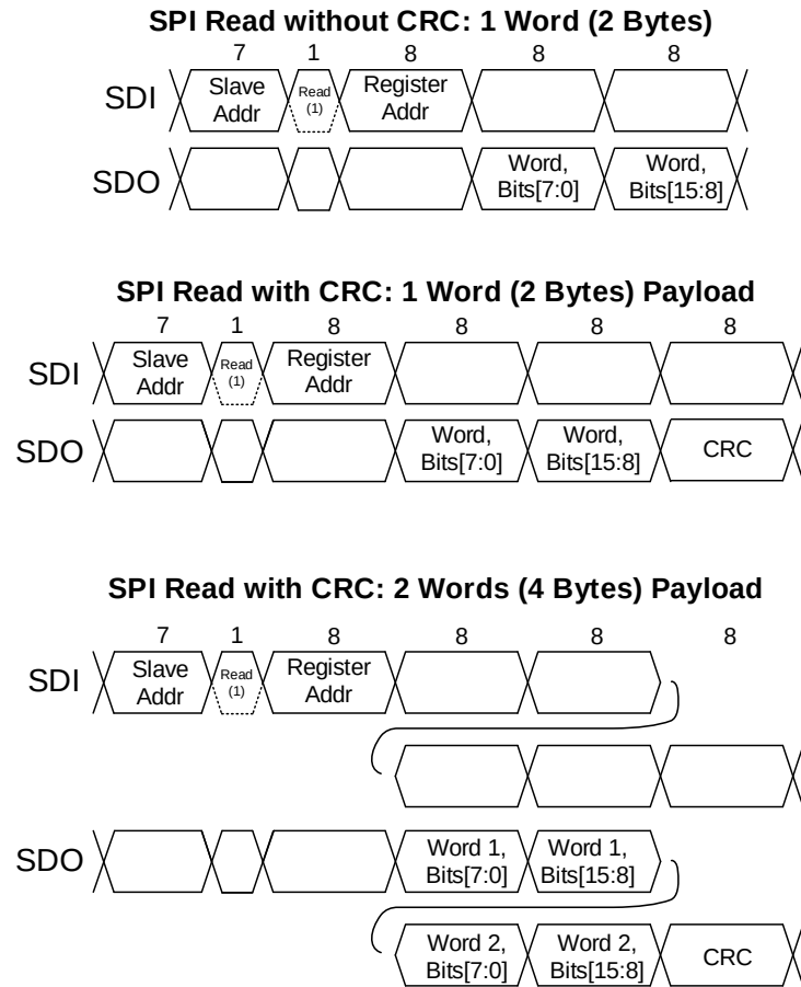
Figure 21: SPI Read Transaction
