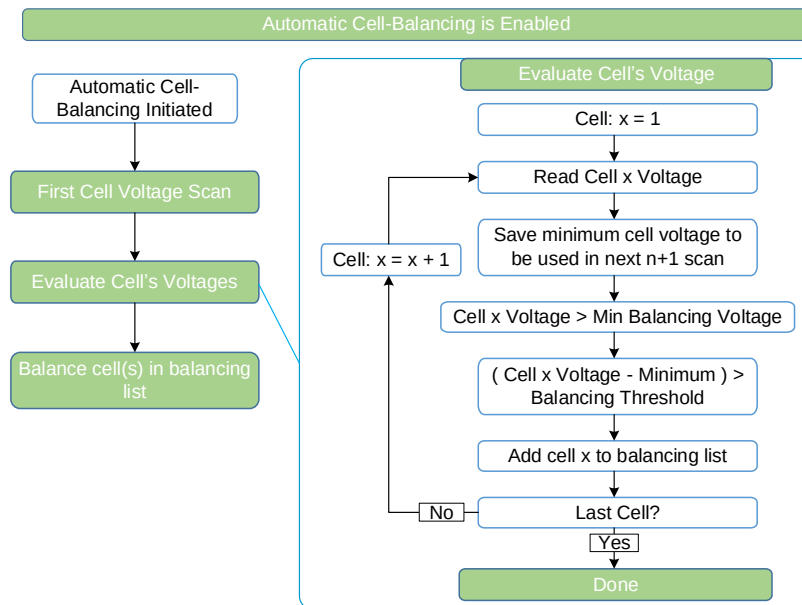
Figure 10: Automatic Cell-Balancing (Cell Voltage Evaluation)
