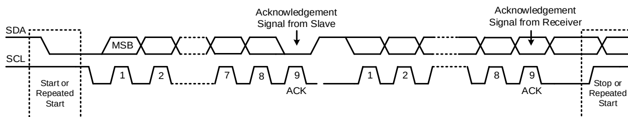
Figure 17: Data Transfer on the I 2 C Bus
