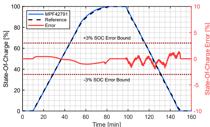
Figure 4: Combined MP2793 + MPF42791 Performance for a CC/CV Charge and Dynamic Discharge (Ambient Temperature = 25°C)
