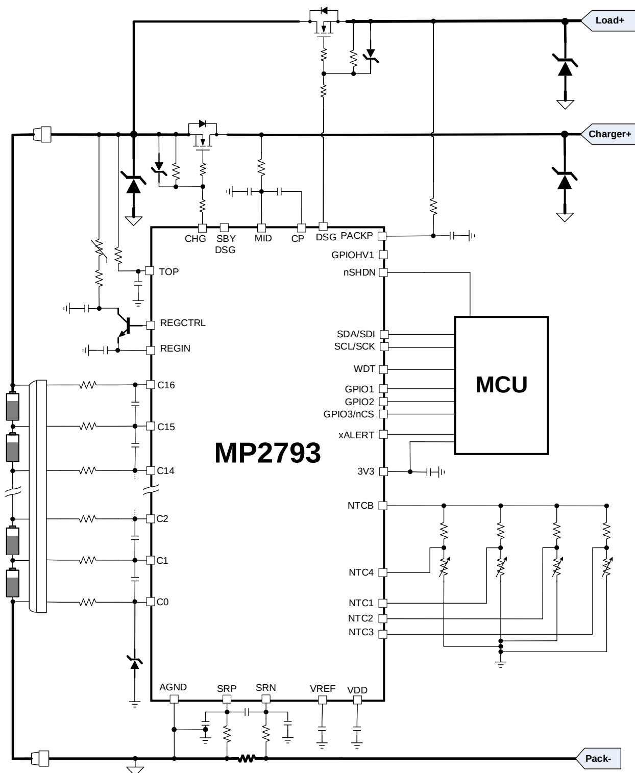
Figure 27: Separate Port Application Circuit for the MP2793
