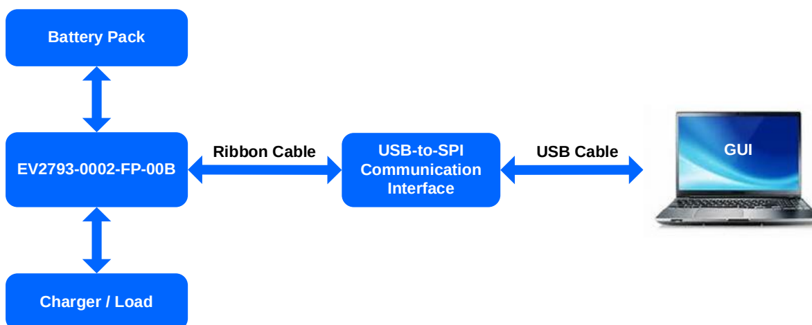
Figure 2: EV2793-0002-FP-00B Evaluation Kit Set-Up
