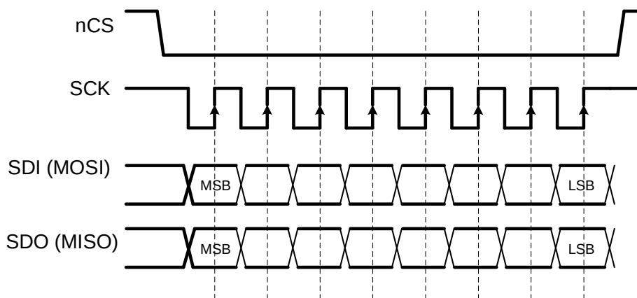
Figure 20: SPI Signal Sequencing
