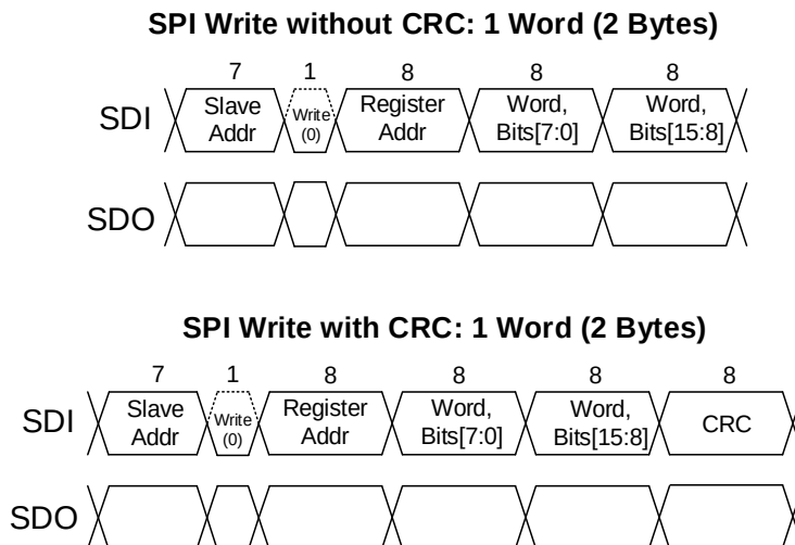
Figure 22: SPI Write Transaction
