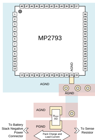
Figure 23: Recommended Layout for AGND
