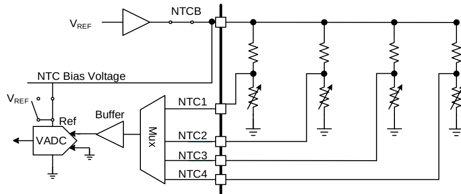
Figure 13: Architecture for NTC ADC Acquisition
