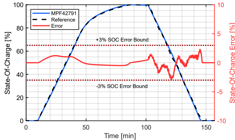
Figure 5: Combined MP2793+MPF42791 Performance for a CC/CV Charge and Dynamic Discharge (Ambient Temperature = 0°C)
