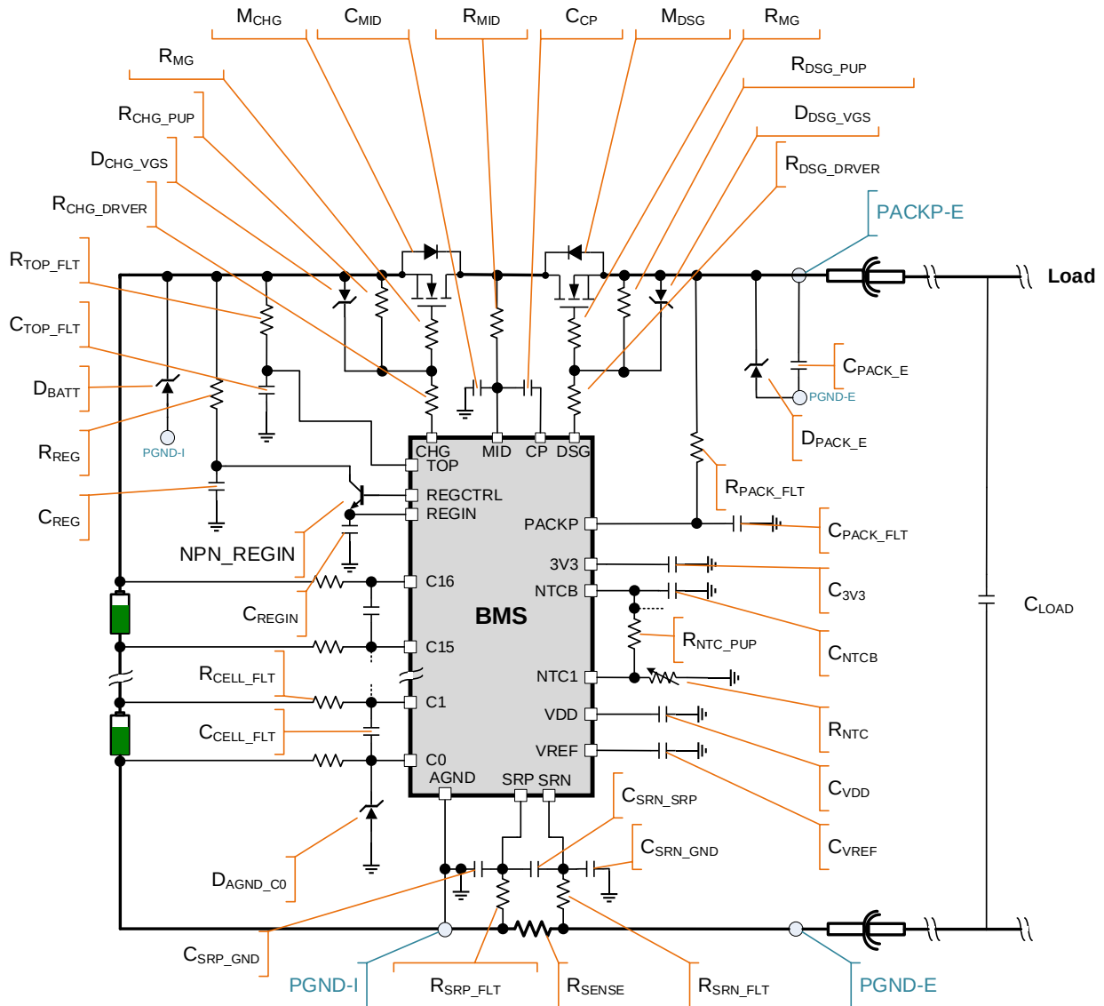
Figure 28: Recommended External Component Diagram
