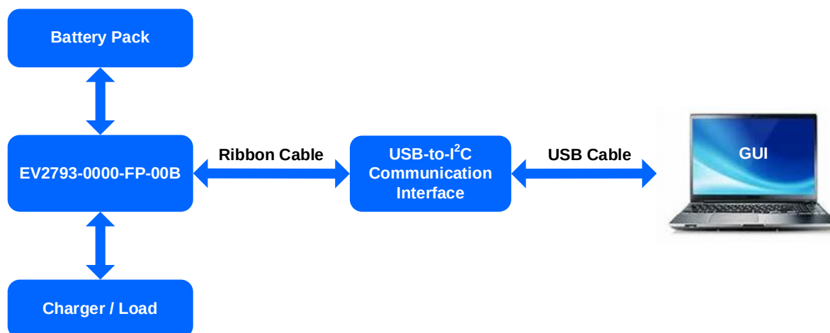
Figure 1: EV2793-0000-FP-00B Evaluation Kit Set-Up
