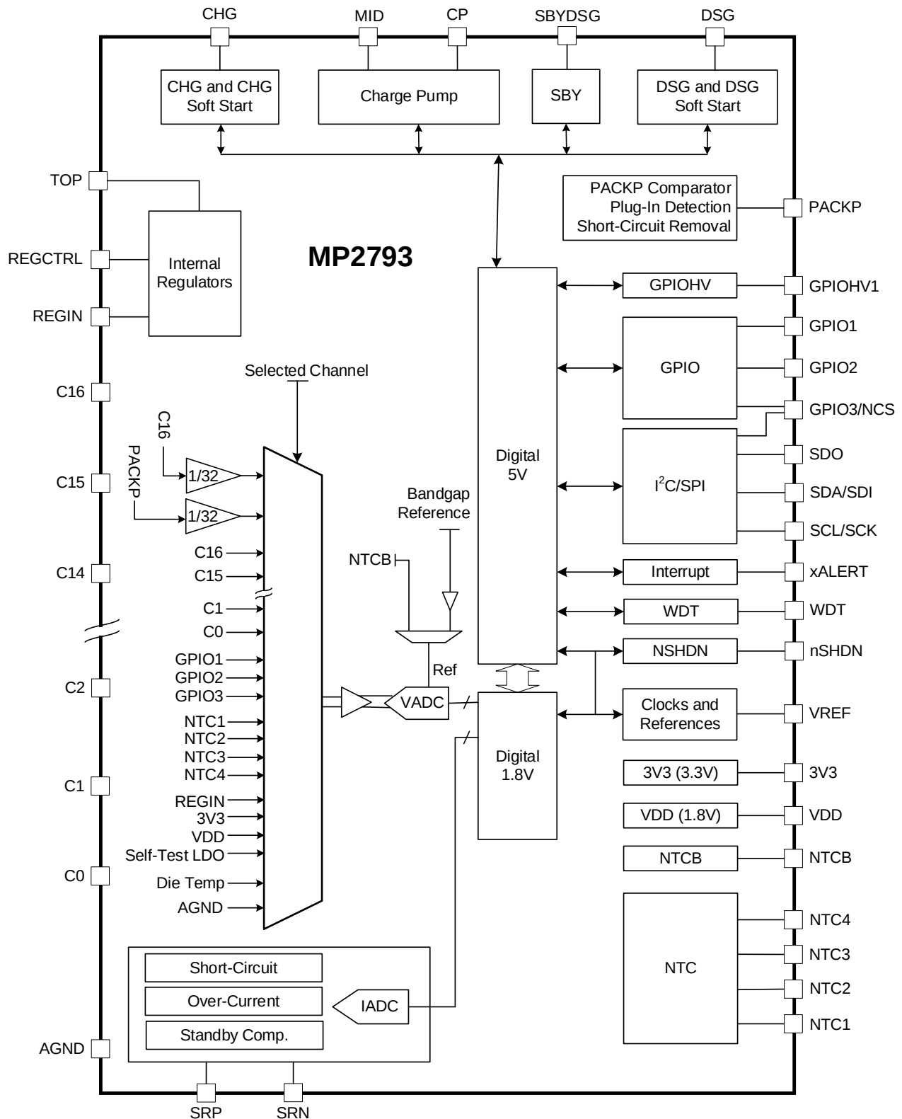
Figure 7: Functional Block Diagram
