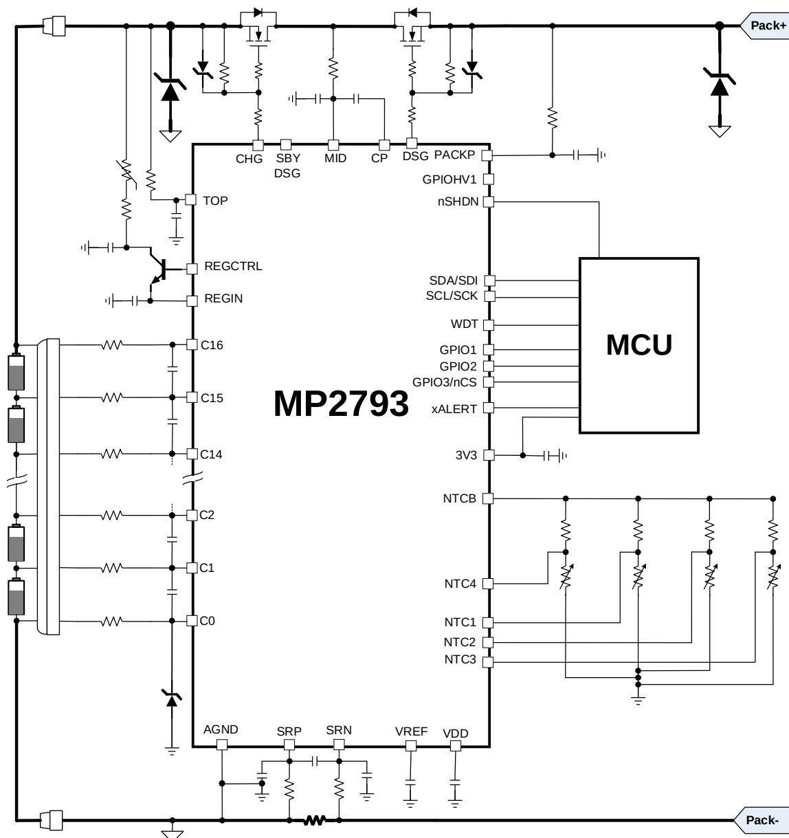
Figure 26: One Port Application Circuit for the MP2793
