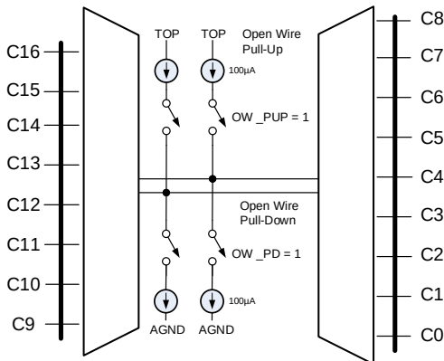
Figure 11: Open-Wire Detection Architecture
