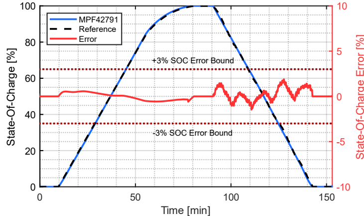
Figure 6: Combined MP2793 + MPF42791 Performance for a CC/CV Charge and Dynamic Discharge (Ambient Temperature = 40°C)
