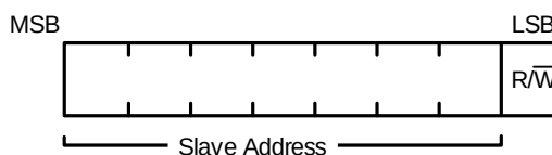
Figure 16: 7-Bit Address
