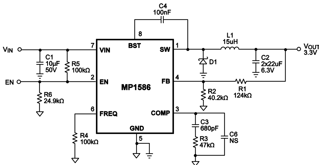
Figure 4—3.3V Output Typical Application Schematic
