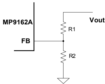
Figure 2: Feedback Network
