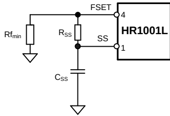
Figure 4: Soft-Start Block
