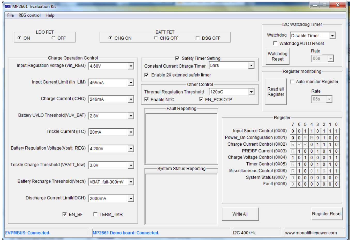
Figure6 MP2661evaluation software
