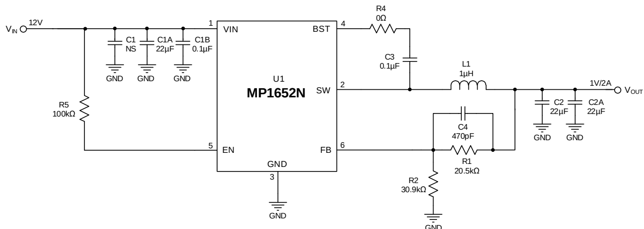
Figure 14: Typical Application Circuit ( V_{IN} = 12V , V_{OUT} = 1V/2A )
