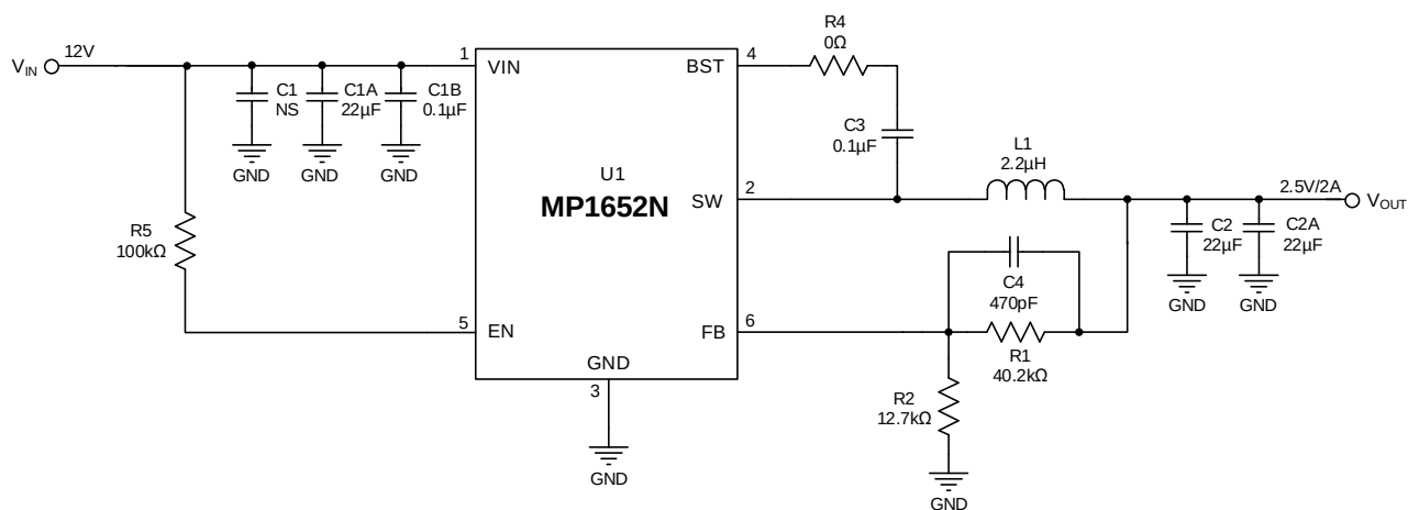
Figure 10: Typical Application Circuit ( V_{IN} = 12V , V_{OUT} = 2.5V/2A )
