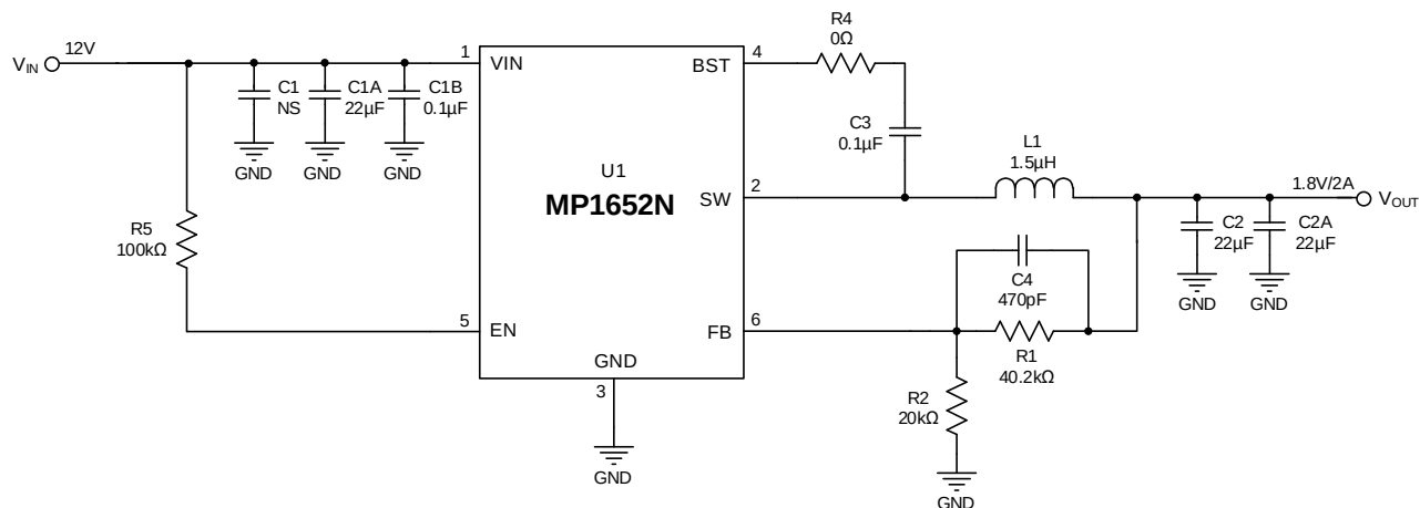
Figure 11: Typical Application Circuit ( V_{IN} = 12V , V_{OUT} = 1.8V/2A )
