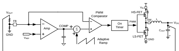
Figure 2: COT Control
