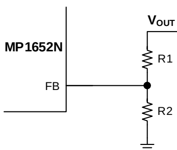
Figure 6: Feedback Network
