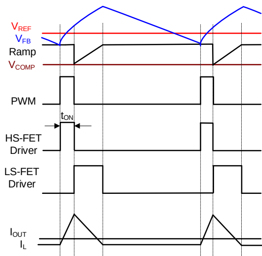
Figure 4: Power-Save Mode at Light Loads
