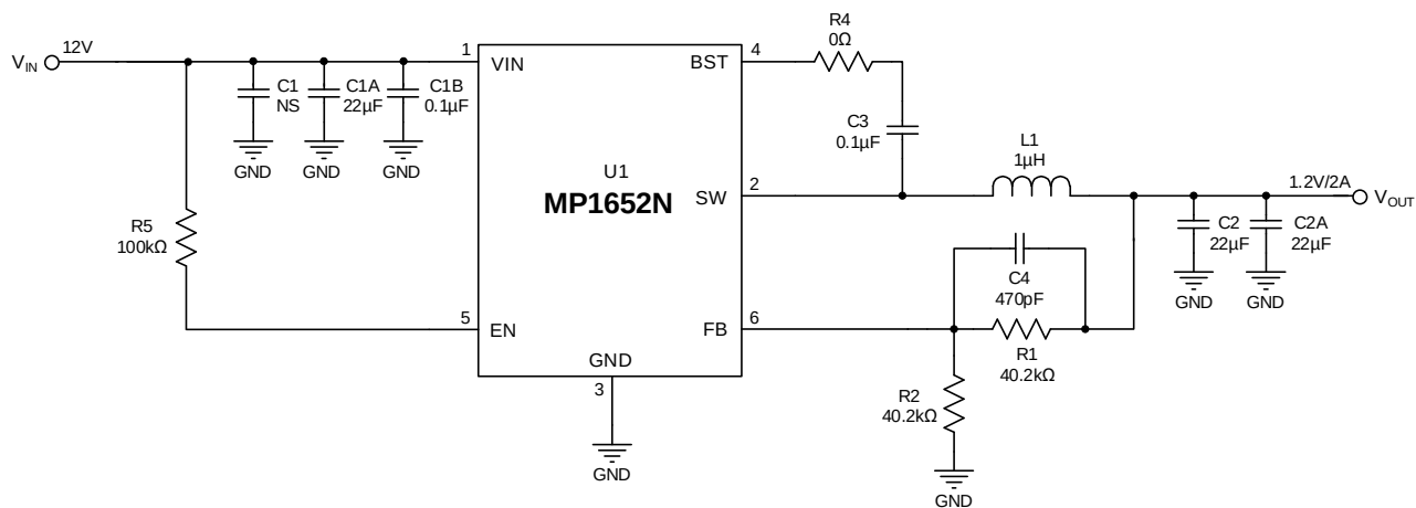
Figure 13: Typical Application Circuit ( V_{IN} = 12V , V_{OUT} = 1.2V/2A )
