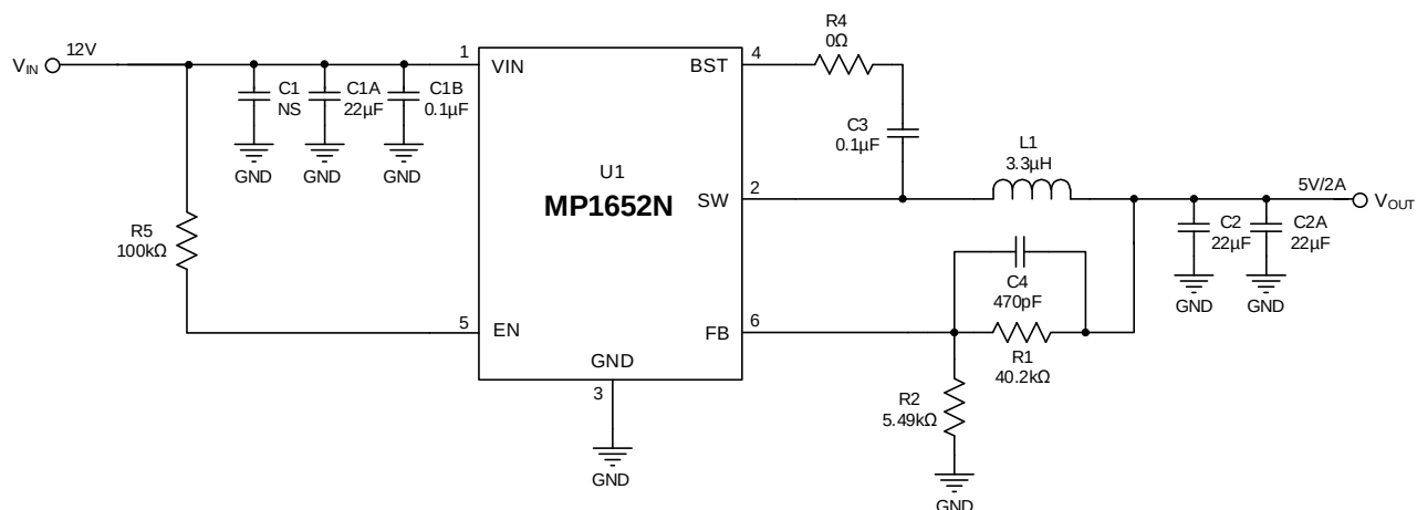
Figure 8: Typical Application Circuit ( V_{IN} = 12V , V_{OUT} = 5V/2A )
