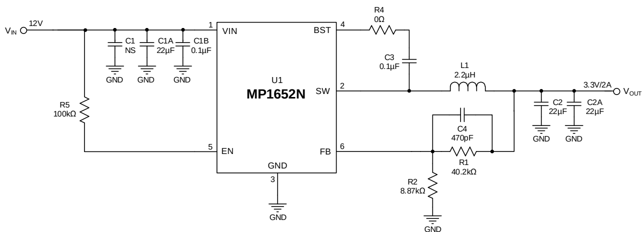
Figure 9: Typical Application Circuit ( V_{IN} = 12V , V_{OUT} = 3.3V/2A )
