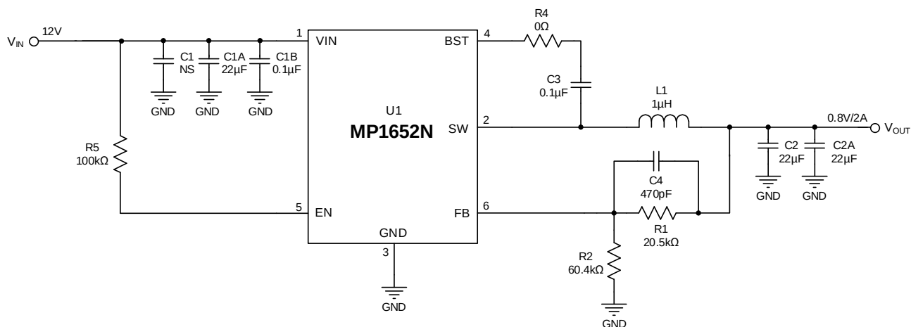
Figure 15: Typical Application Circuit ( V_{IN} = 12V , V_{OUT} = 0.8V/2A )
