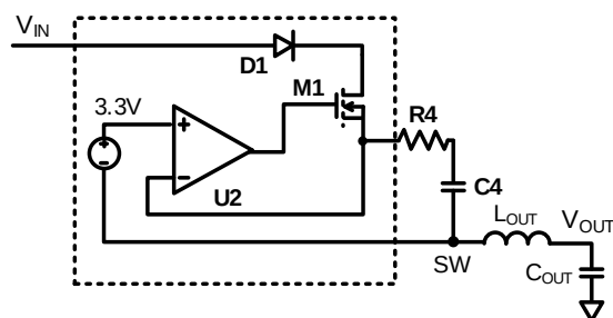
Figure 5: Internal Bootstrap Charger
