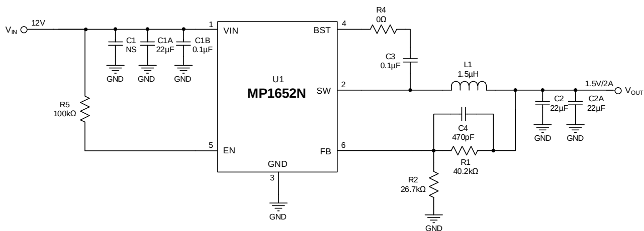
Figure 12: Typical Application Circuit ( V_{IN} = 12V , V_{OUT} = 1.5V/2A )
