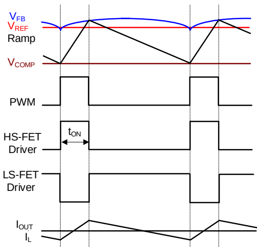
Figure 3: Heavy-Load Operation
