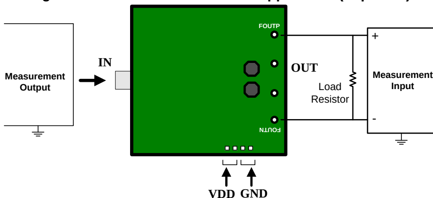
Figure 5—Connection for Normal Application (Top View)
