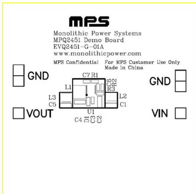
Figure 2—Top and Silk Layer
