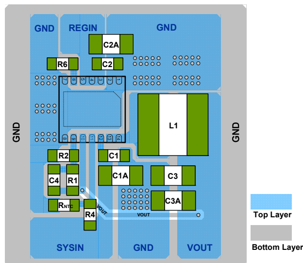
Figure 2: PCB Layout
