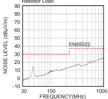
EMI Radiation
