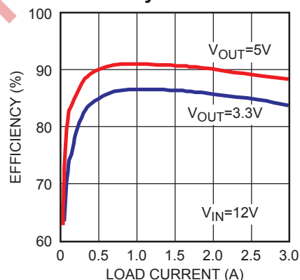
Efficiency Curve
