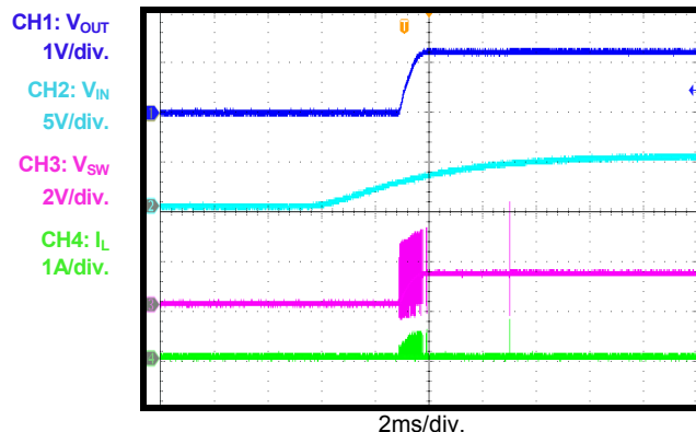
V_{IN} Power-Up
