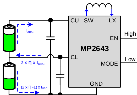
Figure 3: Buck-Balance Mode
