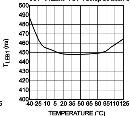
Leading-Edge Blanking for VILIM vs. Temperature
