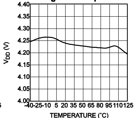
FB Internal Pull-up Voltage vs. Temperature
