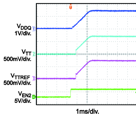
VTT Start-Up through EN2 I_{VDDQ} = I_{VTT} = I_{VTTREF} = 0\text{ A}
