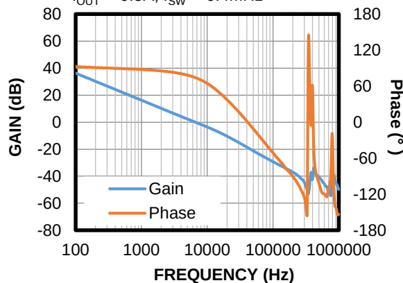
Bode Plot
