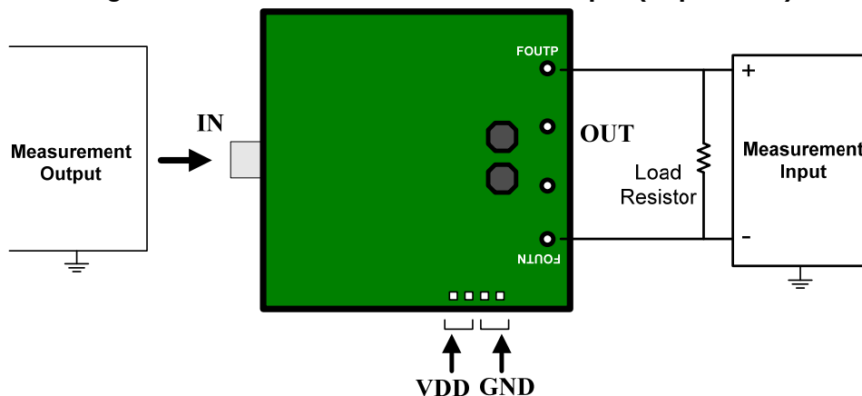
Figure 5—Connection for Mono BTL output (Top viewer)
