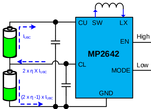
Figure 3: Buck-Balance Mode
