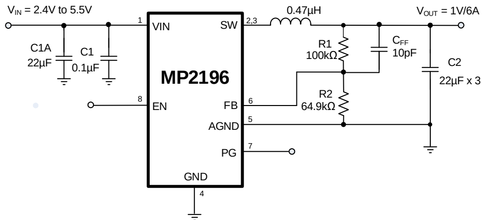
Figure 9: Typical Application Circuit ( V_{IN} = 2.4V to 5.5V , V_{OUT} = 1V/6A )
