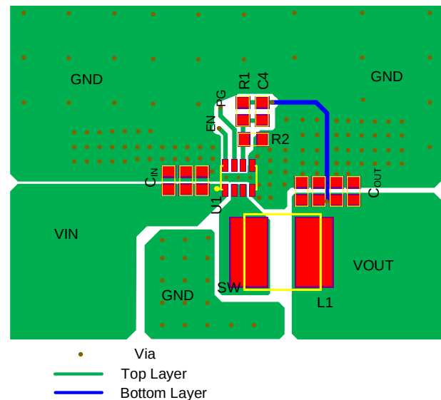
Figure 7: Recommended PCB Layout
