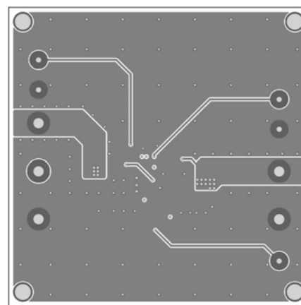
Figure 4 – Inner Layer 2
