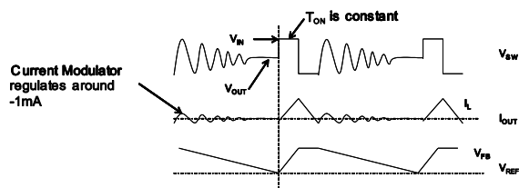
Figure 3: Light-Load Operation
