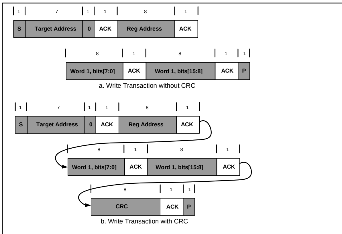
Figure 18: I²C Write Transaction
