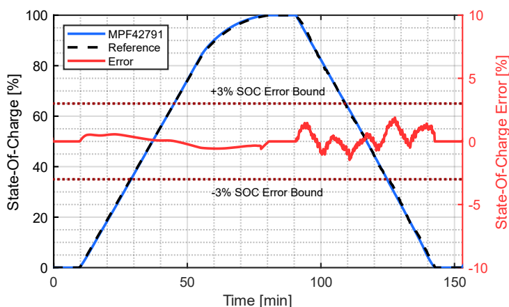
Figure 5: Combined MP2795 + MPF42791 Performance for a CC/CV Charge and Dynamic Discharge (Ambient Temperature = 40°C)
