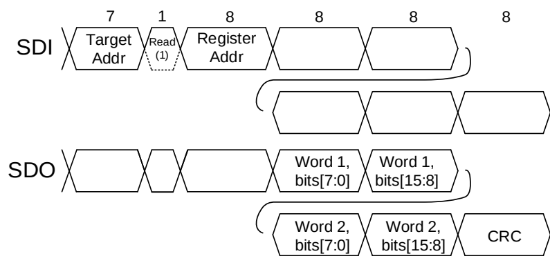
Figure 20: SPI Read Transaction
