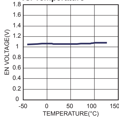
EN Falling Threshold vs. Temperature
