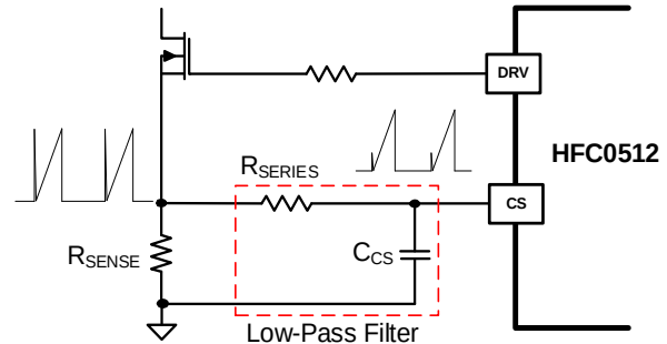
Figure 15: Low-Pass Filter on CS
