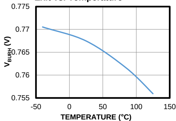
V_{FB} Rising during Burst Mode Exit vs. Temperature
