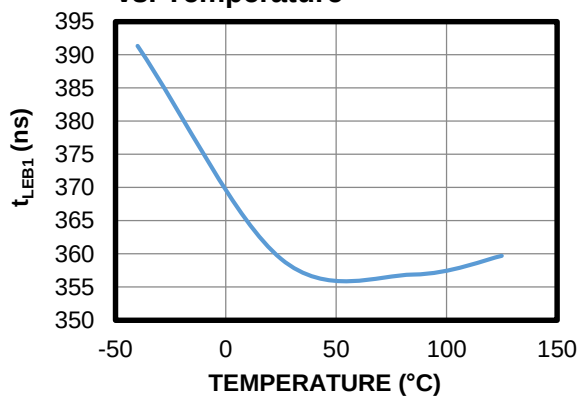
Leading Edge Blanking for V_{ILIMIT} vs. Temperature
