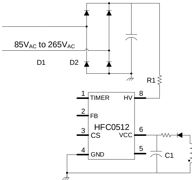
Figure 11: Start-Up Circuit
