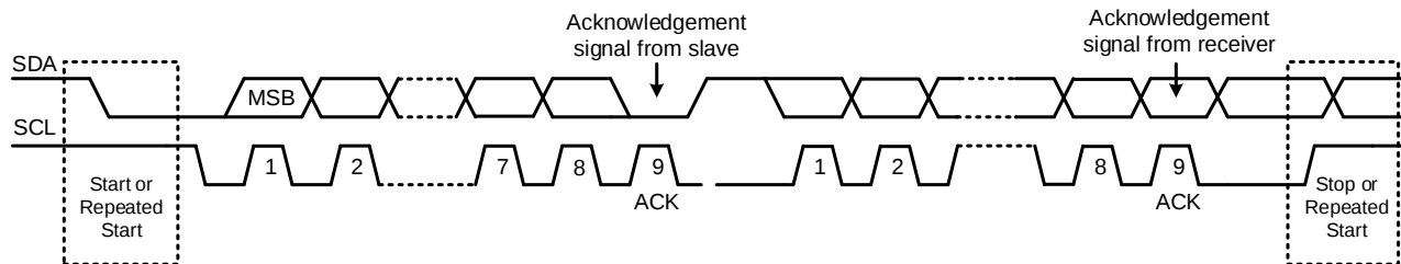
Figure 14: Data Transfer on the I²C Bus
