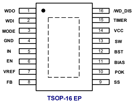
Package Reference
