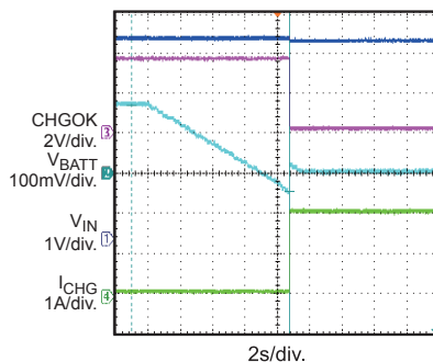
Auto Recharge
