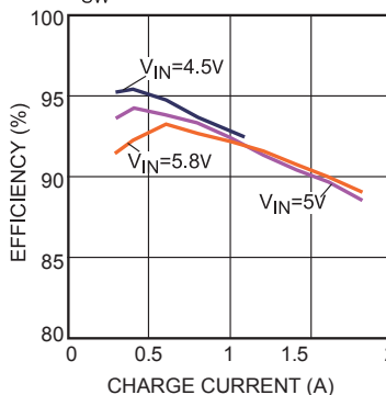
Constant Voltage Charge Efficiency
