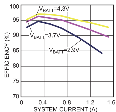
Boost Efficiency
